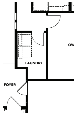
OPT. OWNER'S ENTRY WITH ENLARGED LAUNDRY
