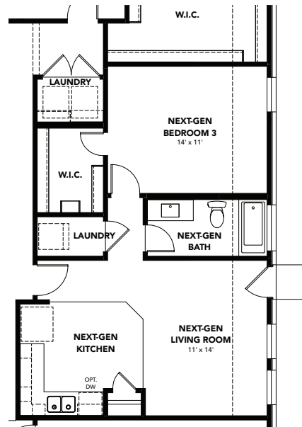
OPT. NEXT-GENERATION SUITE
