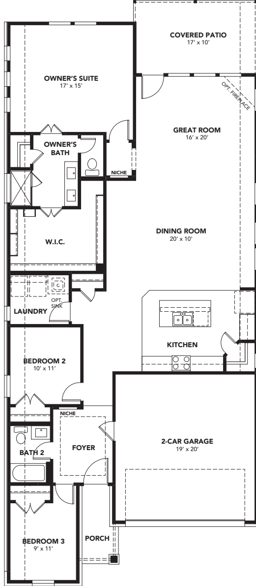
OPT. FIJI PLAN WITH EXTENDED COVERED PATIO
