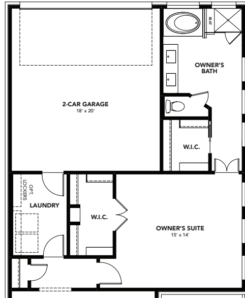
OPT. LUXURY OWNER'S SUITE
