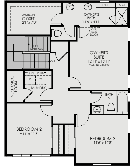
UPPER LEVEL
