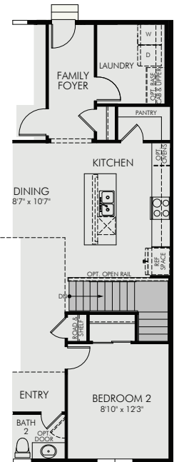
OPT. BASEMENT STAIRS, EXPANDED LAUNDRY
