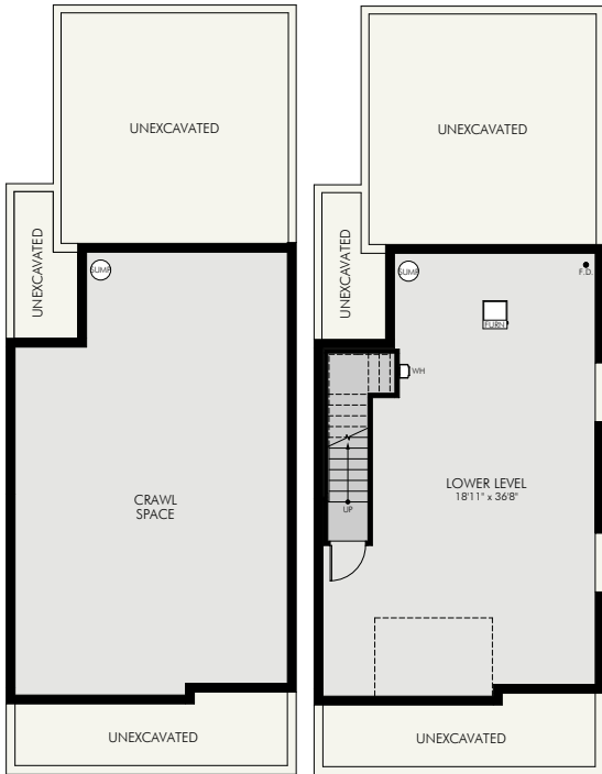
OPT. UNFINISHED LOWER LEVEL
