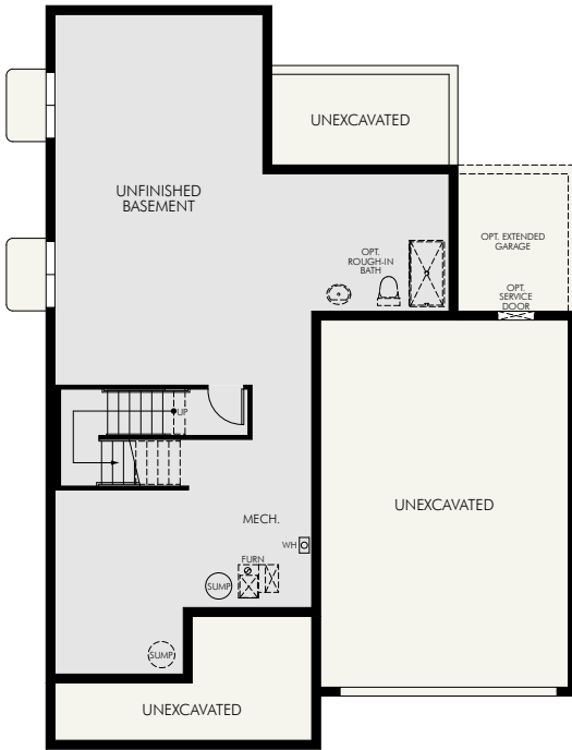
UNFINISHED LOWER LEVEL
