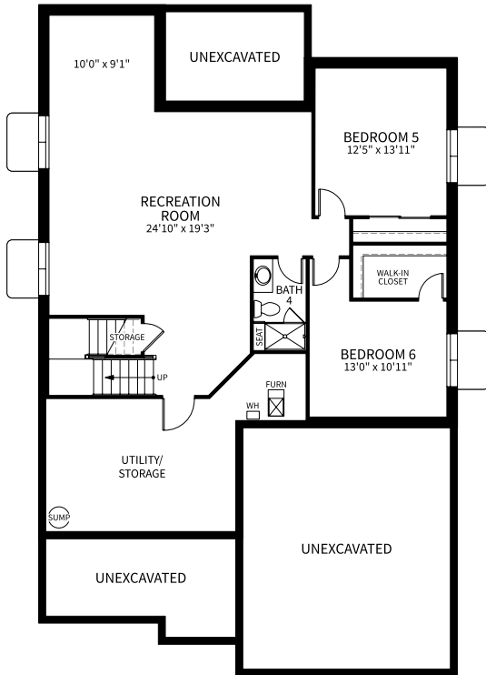
OPT. FINISHED LOWER LEVEL
